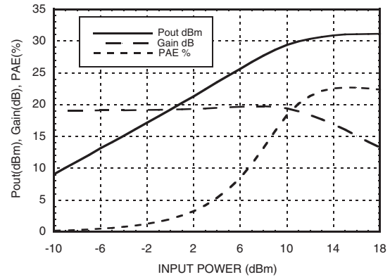
Power Compression @ 30 GHz, 5V @ 800mA
