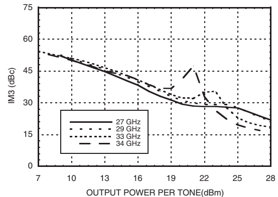
Output IM3, 5V @ 800mA
